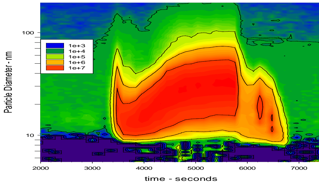
Figure IIIA-14a SMPS spectral content of parked regeneration of 2010 DPF, 2013
