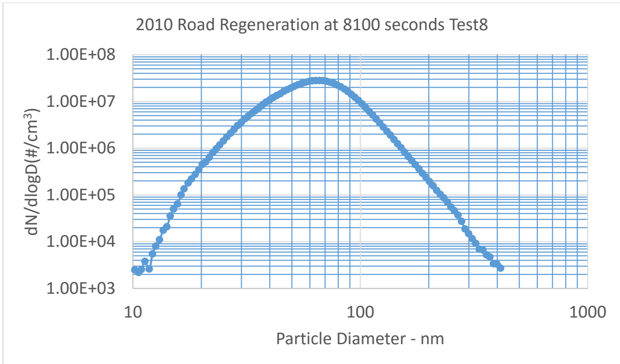
Figure IIIB-18a Normalized particle number concentration at time 8100 seconds, test8
