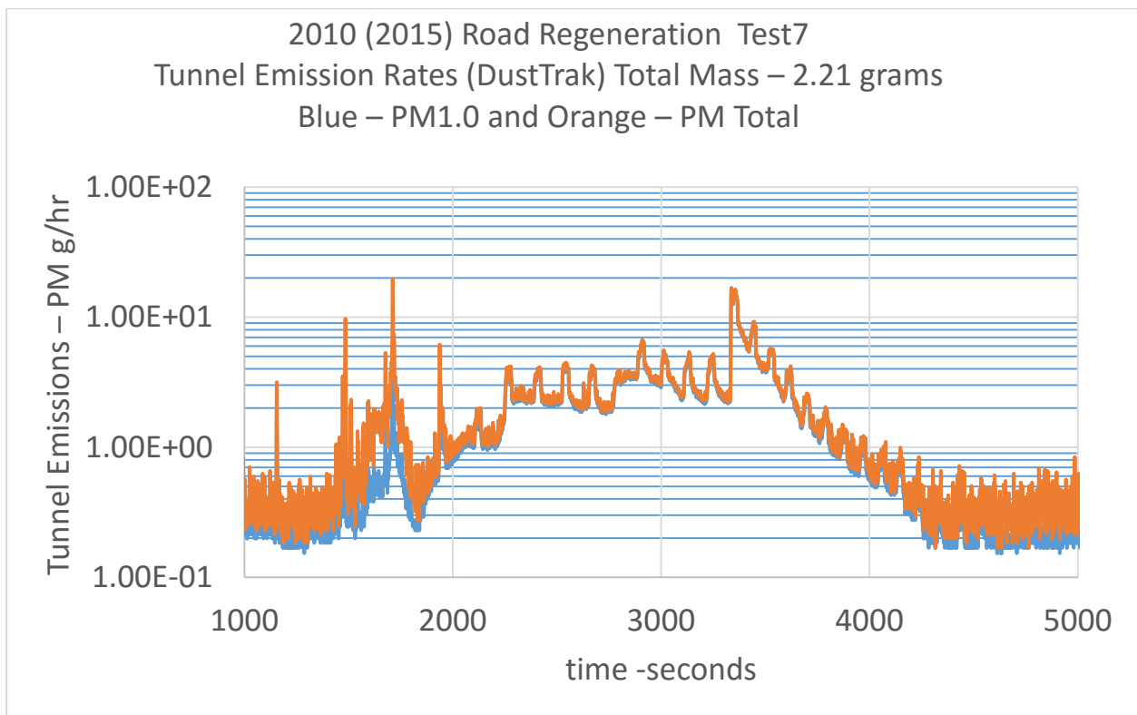
Figure IIIB-12a DustTrak emissions during test7
