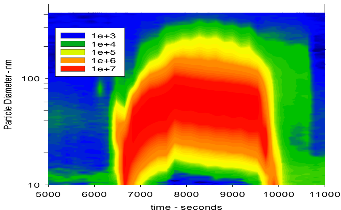
Figure IIIB-14 Normalized spectral particle concentration, test8
