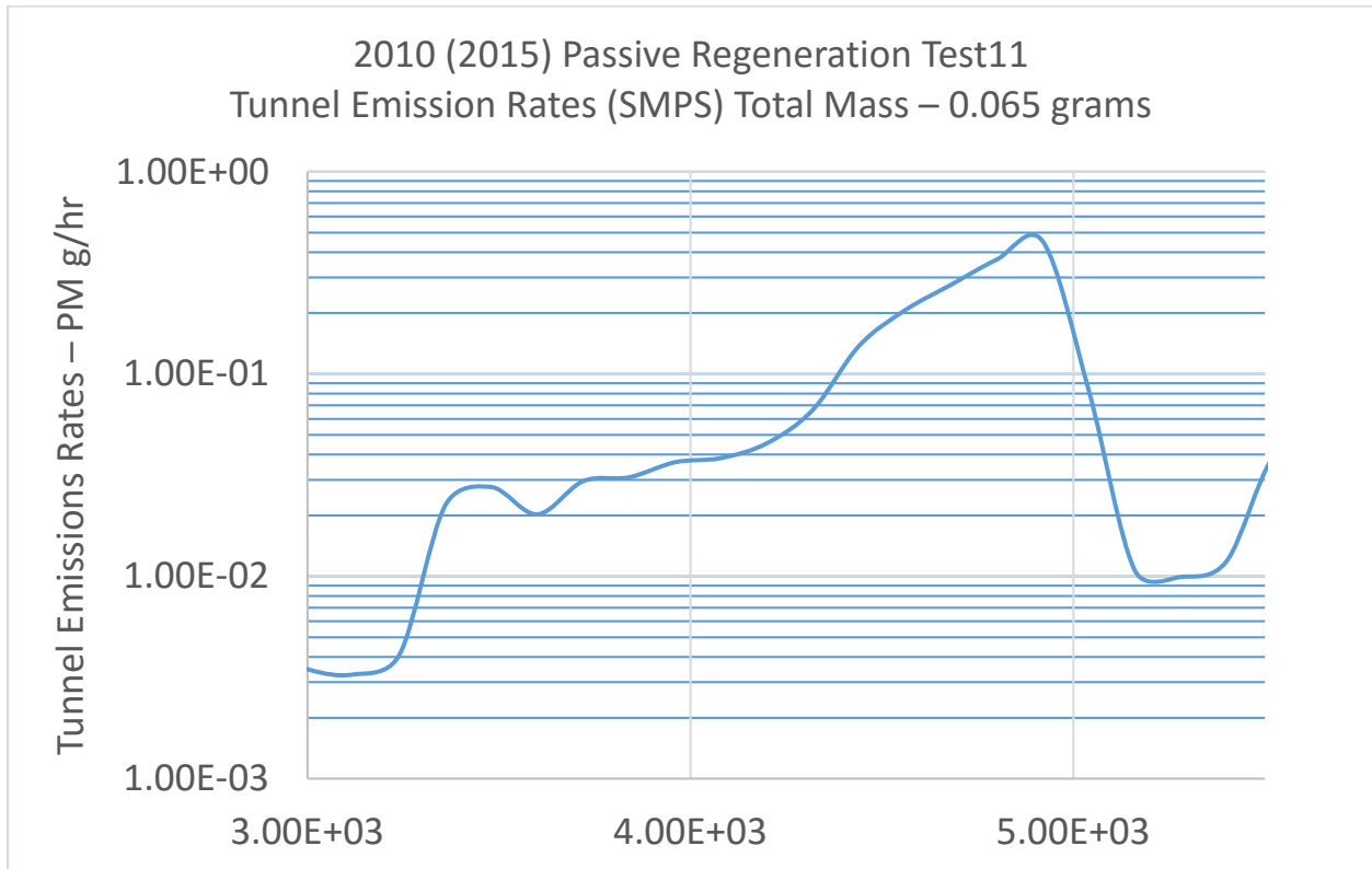
Figure IIC-3 SMPS predicted mass emissions rates during test11
