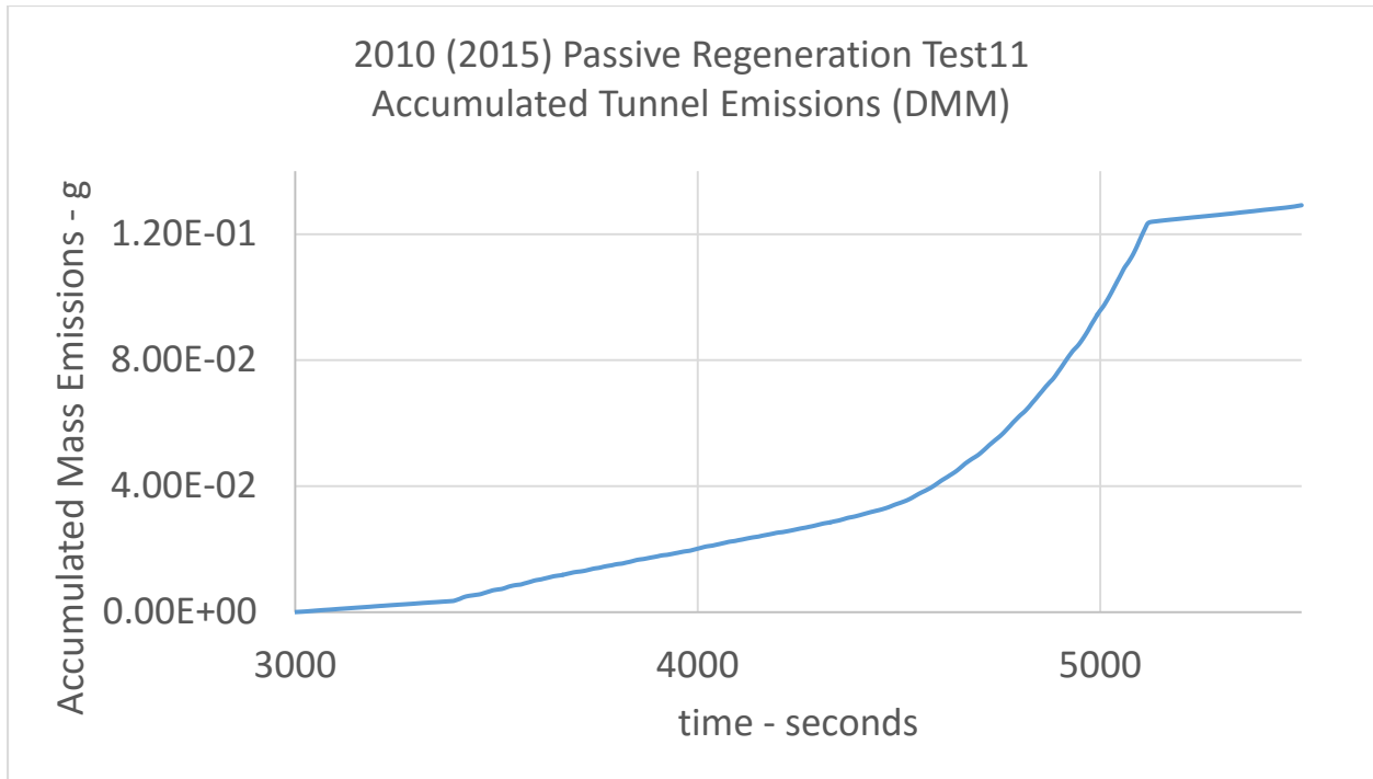
Figure IIC-6 Accumulated mass emission rates for the DMM
