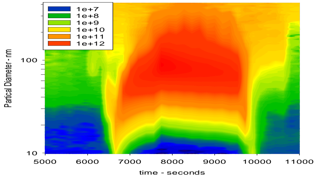
Figure IIIB-16 Normalized volume distribution during test8
