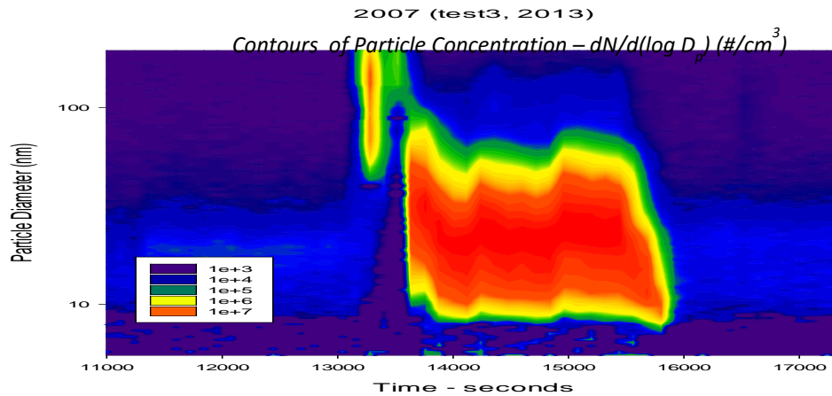
Figure IIIA-3b SMPS spectral emissions, 2013
