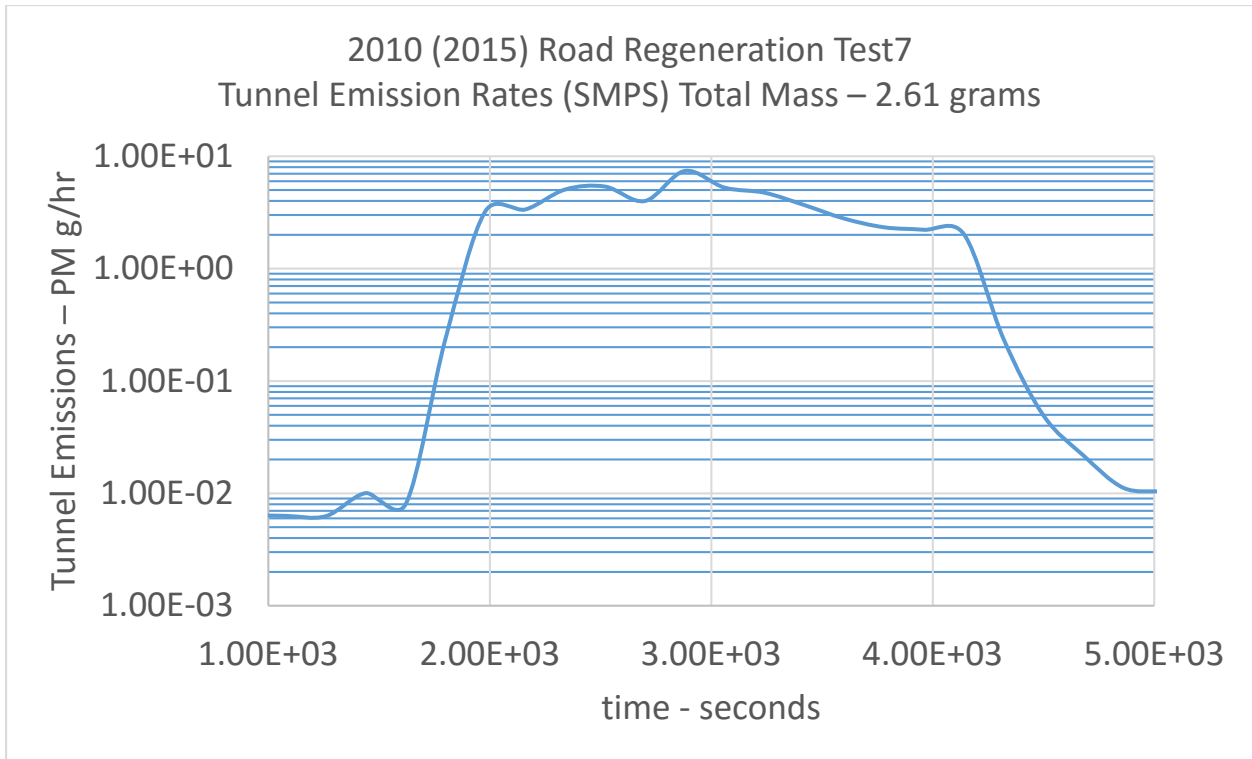
Figure IIIB-10a SMPS mass emission predictions, test7
