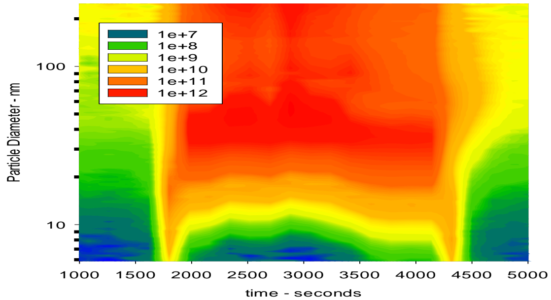
Figure IIIB-15 Normalized volume distribution during test7
