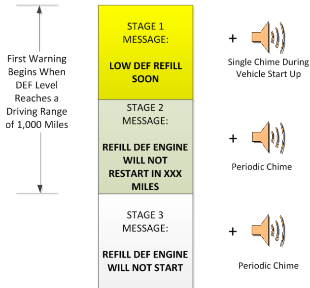
Figure Cummins 6.7-3: 2010 Cummins' 6.7L SCR System DEF Depletion Warning Sequence
