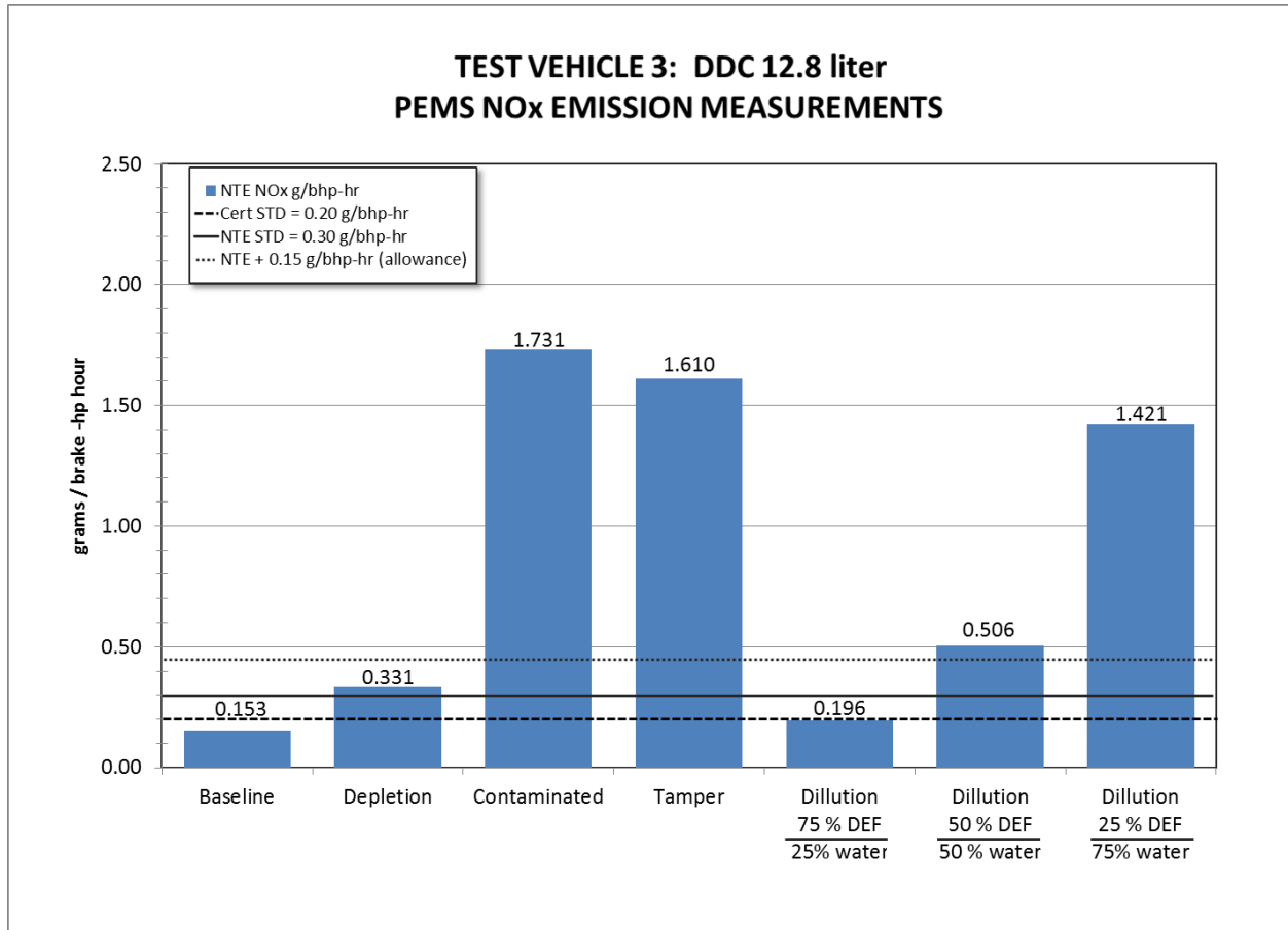
Figure DDC-13: Vehicle 3 - NOx Emission Data Summary
