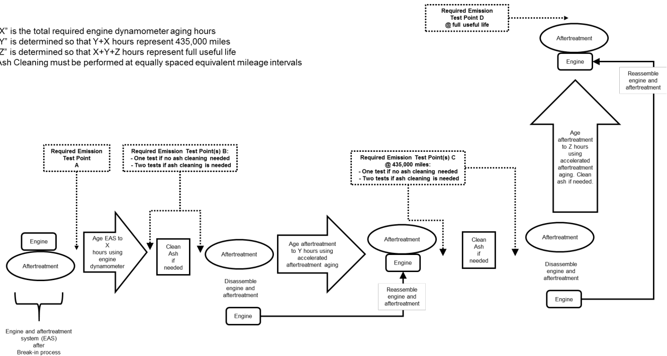
Figure CA26-5: Alternative Durability Demonstration Using Accelerated Aftertreatment Aging for 2027 and Subsequent Model Year Heavy Heavy-Duty Engines
