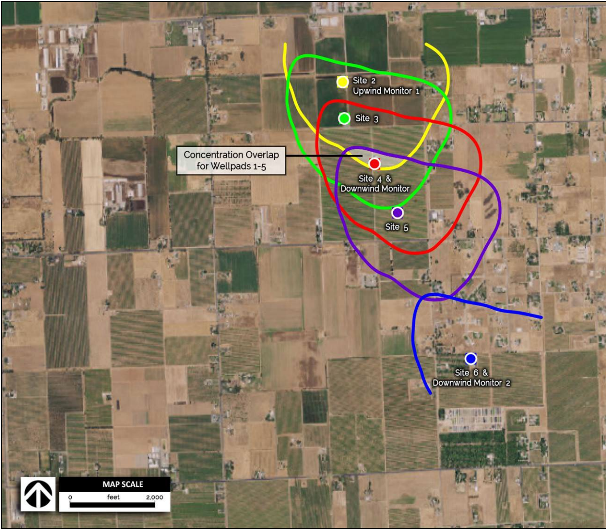
Figure 4: Isopleth Map for Modeled Potential Emissions
